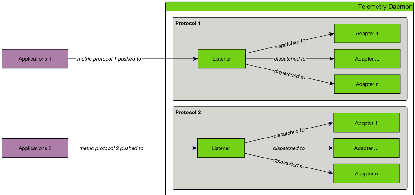
Figure 41. Generic component overview of protocol implementations in Telemetryd
