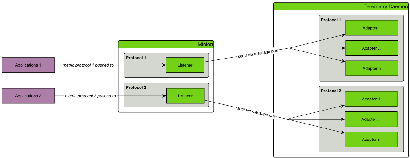
Figure 42. Running Listener on a Minion forwarding packets using the messaging system
