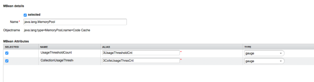
Figure 11. Configure MBean attributes for data collection configuration
